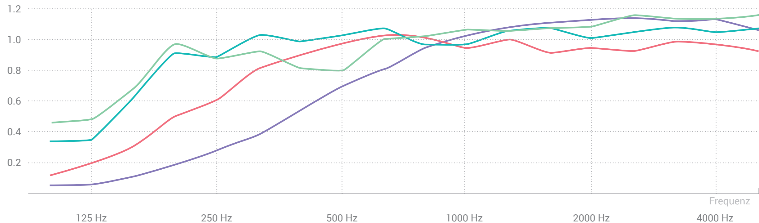
Schallabsorptionsgrad aPerf® 25
